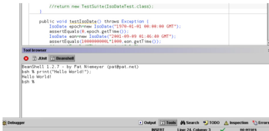
Console Beanshell
