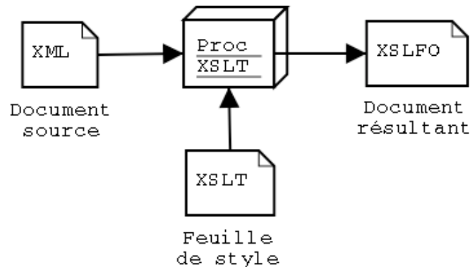
Figure 1: Transformation XSL-FO
